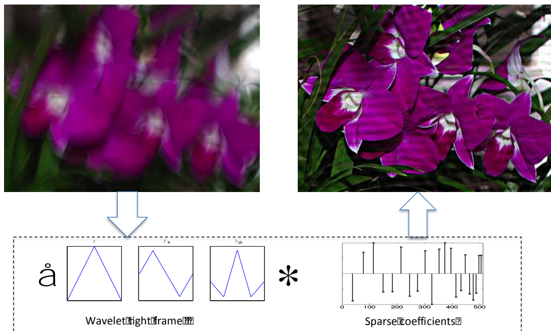
Figure 1. Work flow of blind image deblurring by sparse approximation
